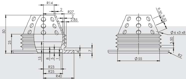
flexi-led vertical lamp holder
