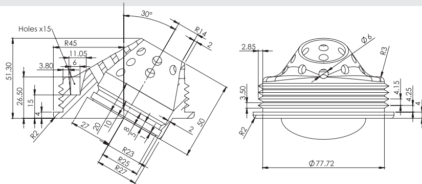
flexi-led directional lamp holder
